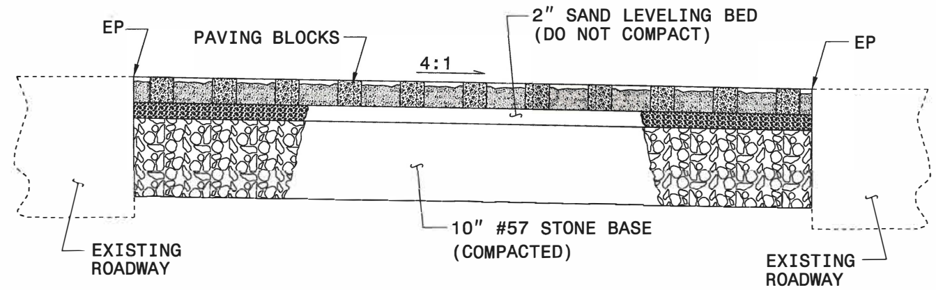
SECTION "A-A"
